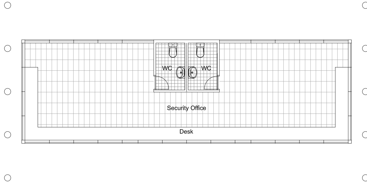
Gatehouse Detail
