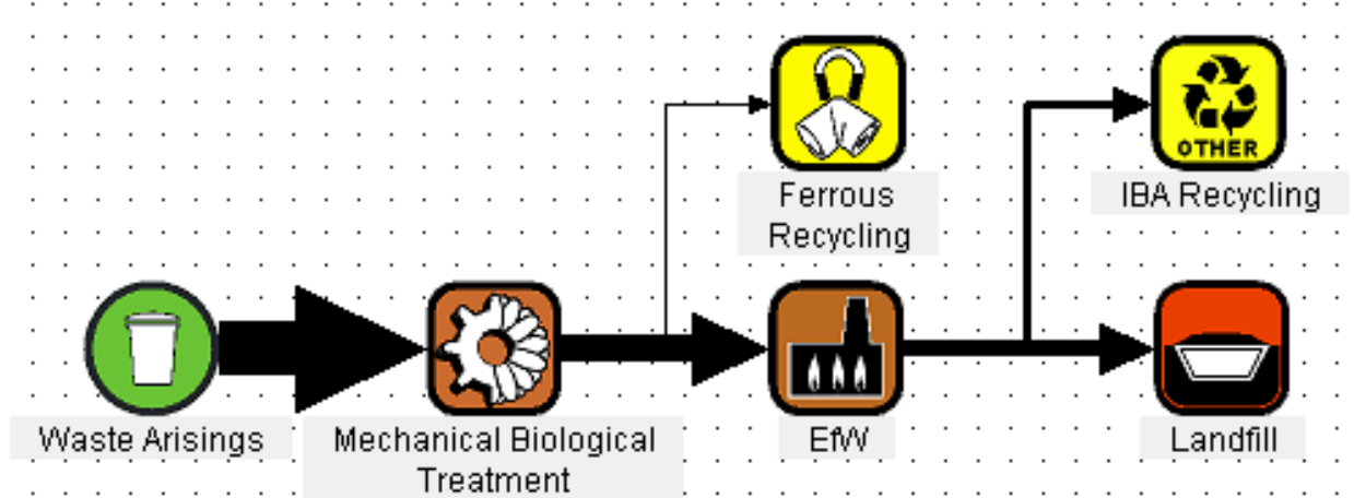
Figure A-4 Mechanical Biological Treatment (MBT) with Refuse Derived Fuel (RDF) going to Energy from Waste (EfW) Sankey Diagram
