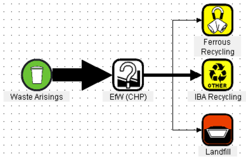
Figure A-3 Energy from Waste (EfW) with Combined Heat and Power Sankey Diagram
