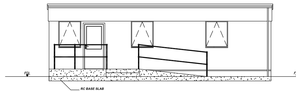
NORTH ELEVATION
